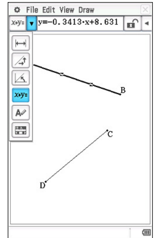
Equation of AB
