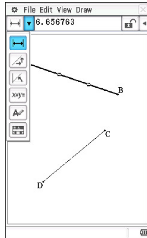
Length of AB
